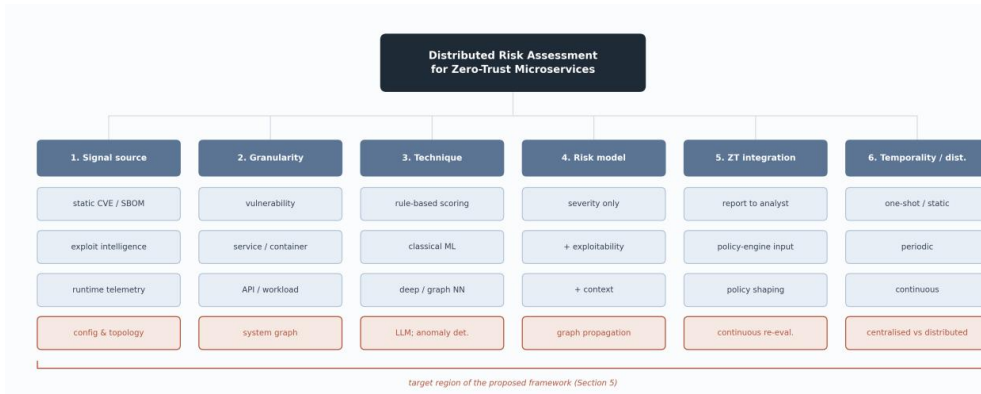
Figure 3 A Six-Dimension Taxonomy of Distributed Risk Assessment for Zero-Trust Microservices
