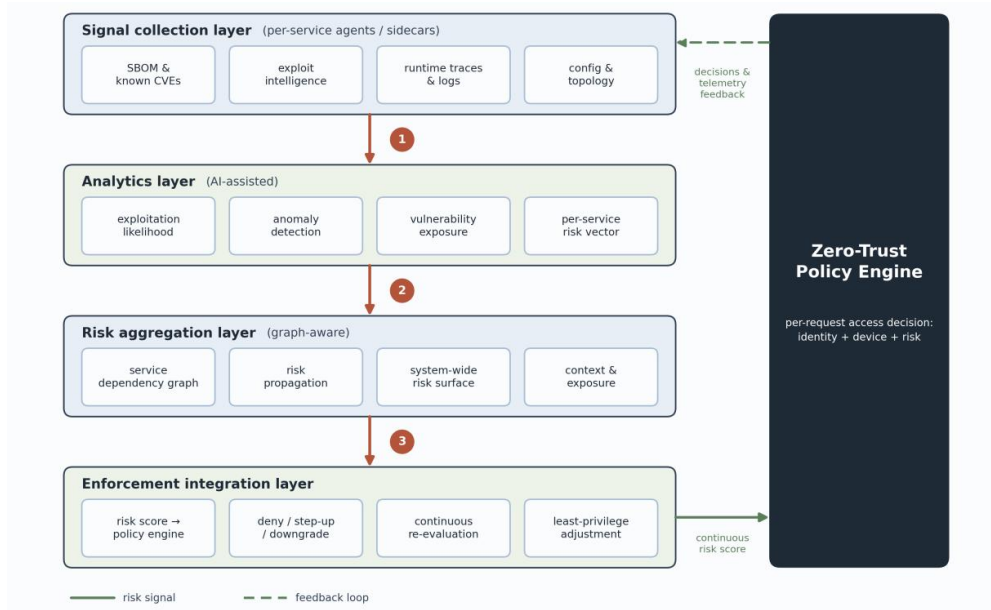
Figure 4 The Four-Layer Conceptual Framework
